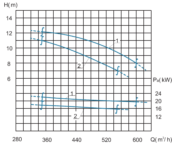
Performance Curve
