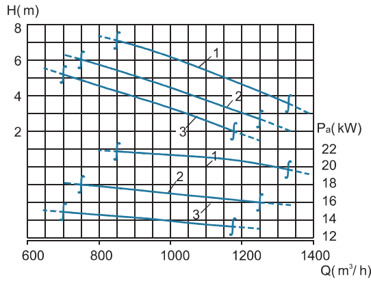
Performance Curve
